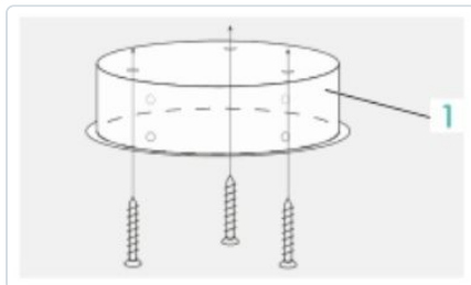
1 Ceiling bracket
